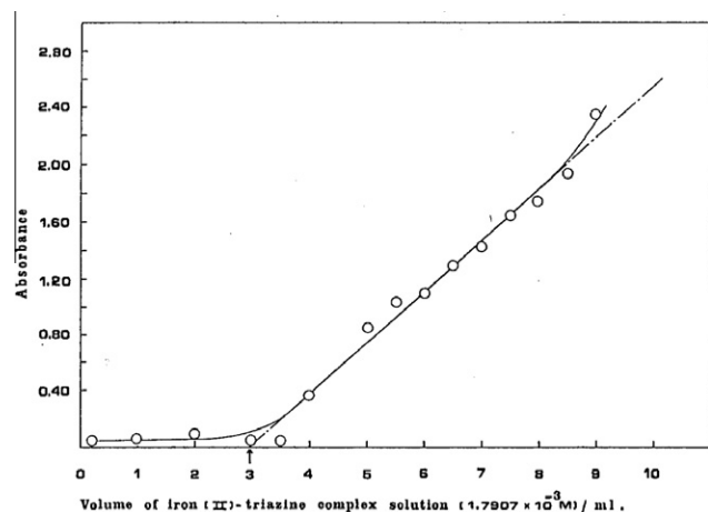
Figure 1 Determination of sorption capacity of iron(II)-triazine on silica gel. 1 g amount of conditioned silica gel; 0.2–10 ml of 1.7907 \times 10^{-3} M \text{Fe}(\text{TPTZ})_2^{2+} solution were added and the volume was made up to 10 ml with distilled water. Shaking time, 20 min. Unadsorbed \text{Fe}(\text{TPTZ})_2^{2+} was measured at 592 nm using 1 cm cell.
