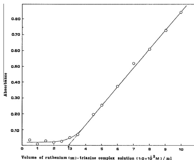
Figure 2 Determination of sorption capacity of ruthenium(III)-triazine on silica gel. 1 g amount of conditioned silica gel; 0.2–10 ml of 1.0 \times 10^{-3} M \text{Ru}(\text{TPTZ})_2^{3+} solution were added and the volume was made up to 10 ml with distilled water. Shaking time, 20 min. Unadsorbed \text{Ru}(\text{TPTZ})_2^{3+} was measured at 510 nm using 1 cm cell.
