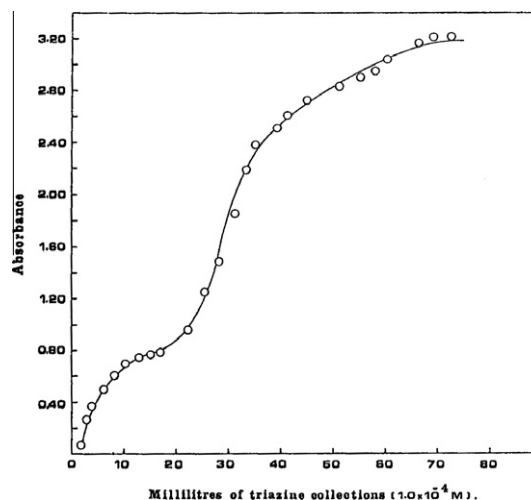
Figure 3 Adsorbability of triazine on silica gel in a small column; TPTZ solution ( 1.0 \times 10^{-4} M in 2.5% ethanol) was passed through at flow rate of 1 ml/min. Absorbance at 285 nm for each 3 ml of the effluent was measured.
